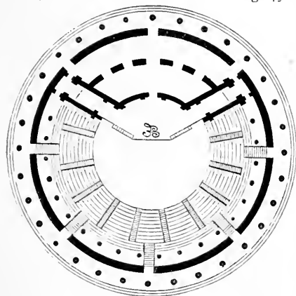
Fig. 496. Ground-plan of the Odeon at Athens.
